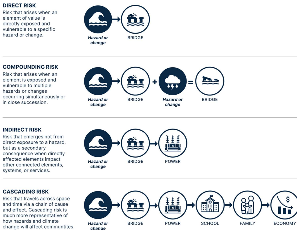
Figure 1. Definition and illustration of direct, compounding, and cascading risk
